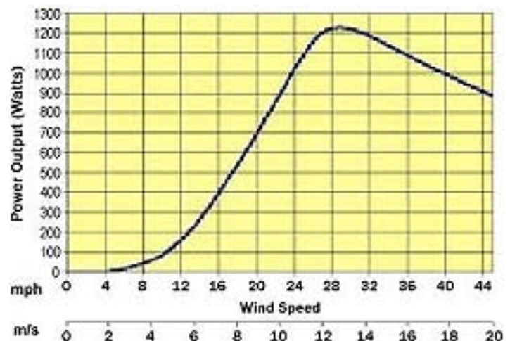
Sample power curve diagram:
